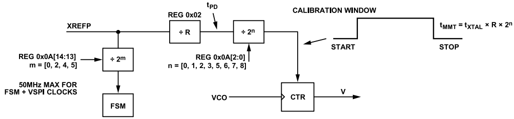
Figure 22. VCO Calibration
