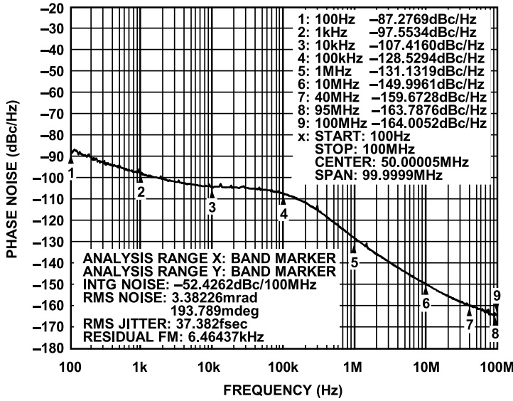
Figure 7. Closed-Loop Phase Noise Illustrating Low Jitter Capability at 14.4 GHz, Wenzel 100 MHz Reference, 100 MHz PFD, RFOUT, High Performance Mode (VCO Register 0x01, Bits[4:2] = 7 (Decimal)), 25°C
