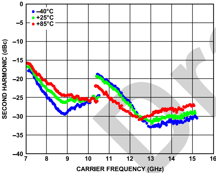
Figure 12. Second Harmonic vs. Carrier Frequency at RFOUT, Maximum Output Gain (VCO Register 0x01, Bits[1:0] = 3 (Decimal)), High Performance Mode (VCO Register 0x01, Bits[4:2] = 7 (Decimal))
