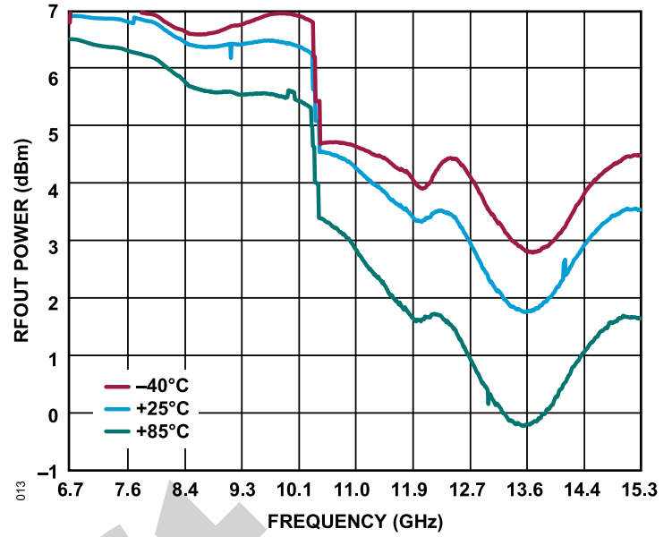
Figure 9. RFOUT Power vs. Carrier Frequency, Maximum Output Gain = (VCO Register 0x01, Bits[1:0] = 3 (Decimal)), High Performance Mode (VCO Register 0x01, Bits[4:2] = 7 (Decimal))
