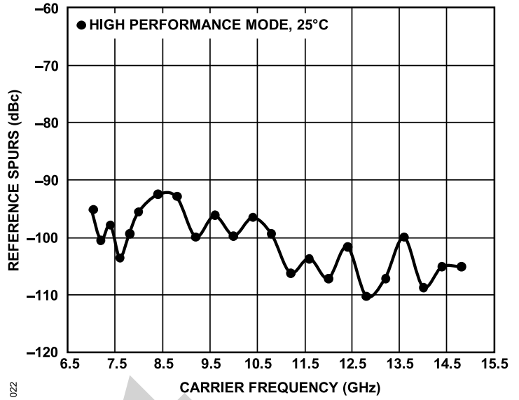
Figure 17. Reference Spurs vs. Carrier Frequency, 100 MHz PFD Frequency, Maximum Output Gain (VCO Register 0x01, Bits[1:0] = 3 (Decimal)), High Performance Mode (VCO Register 0x01, Bits[4:2] = 7 (Decimal))
