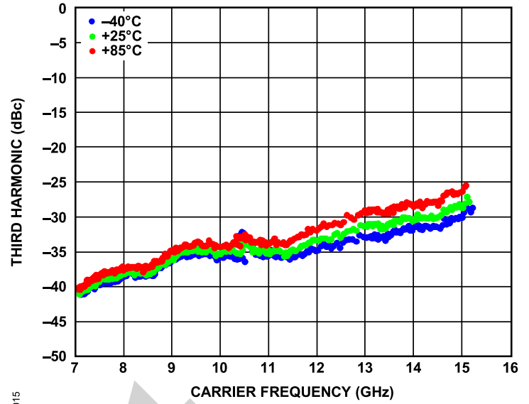
Figure 13. Third Harmonic vs. Carrier Frequency, Maximum Output Gain (VCO Register 0x01, Bits[1:0] = 3 (Decimal)), High Performance Mode (VCO Register 0x01, Bits[4:2] = 7 (Decimal))
