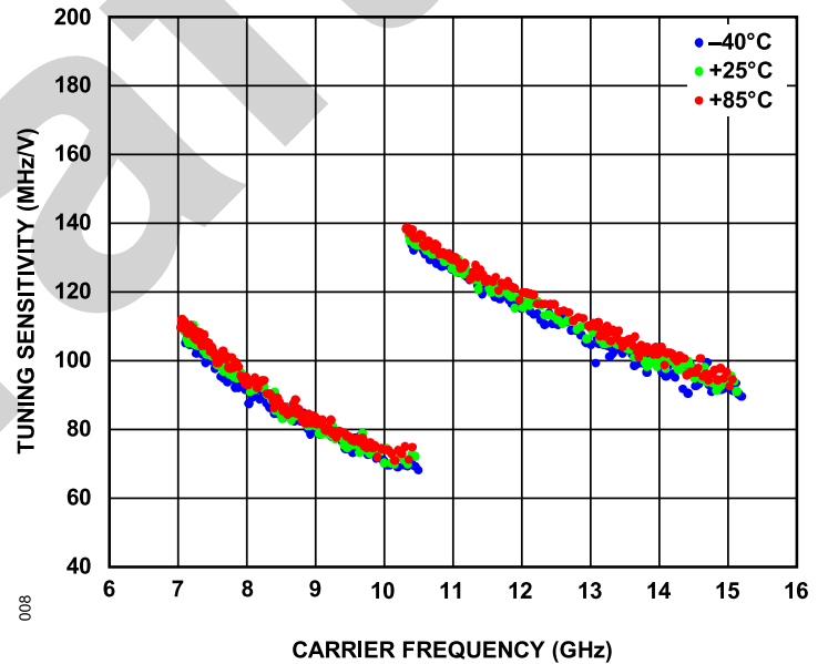
Figure 10. Tuning Sensitivity vs. Carrier Frequency, VT = 1.65 V, Maximum Output Gain (VCO Register 0x01, Bits[1:0] = 3 (Decimal)), High Performance Mode (VCO Register 0x01, Bits[4:2] = 7 (Decimal))
