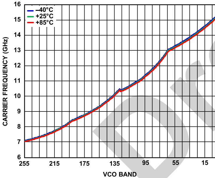
Figure 8. Carrier Frequency vs. VCO Band, Autocalibration Enabled, VDDLs = 3.3 V, VPPCP = 3.3 V
