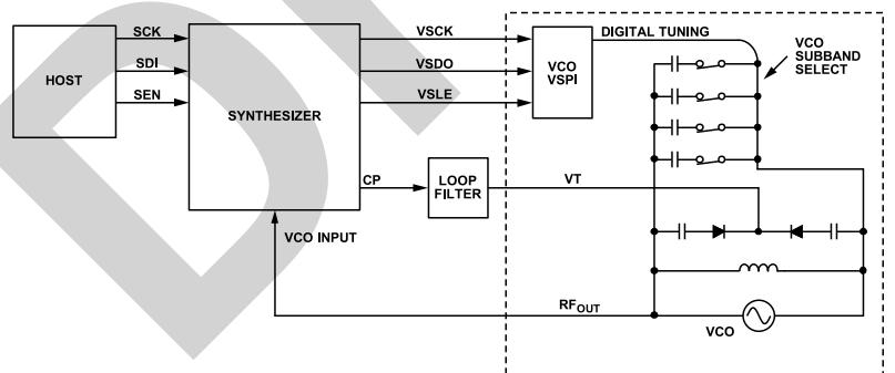
Figure 20. Simplified Step Tuned VCO
